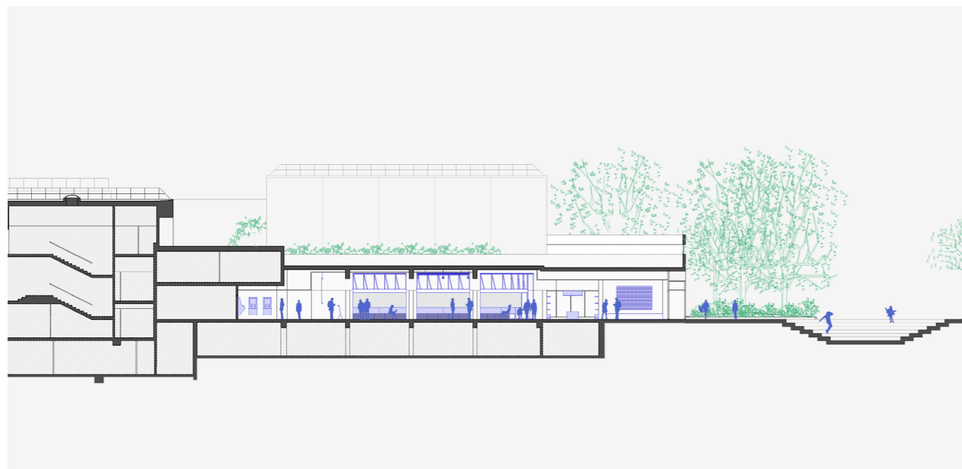
Coupe longitudinale du rez-de-chaussée de l'occupation temporaire, 2024 | © SAME Ground floor longitudinal section of the temporary occupation, 2024 | © SAME
