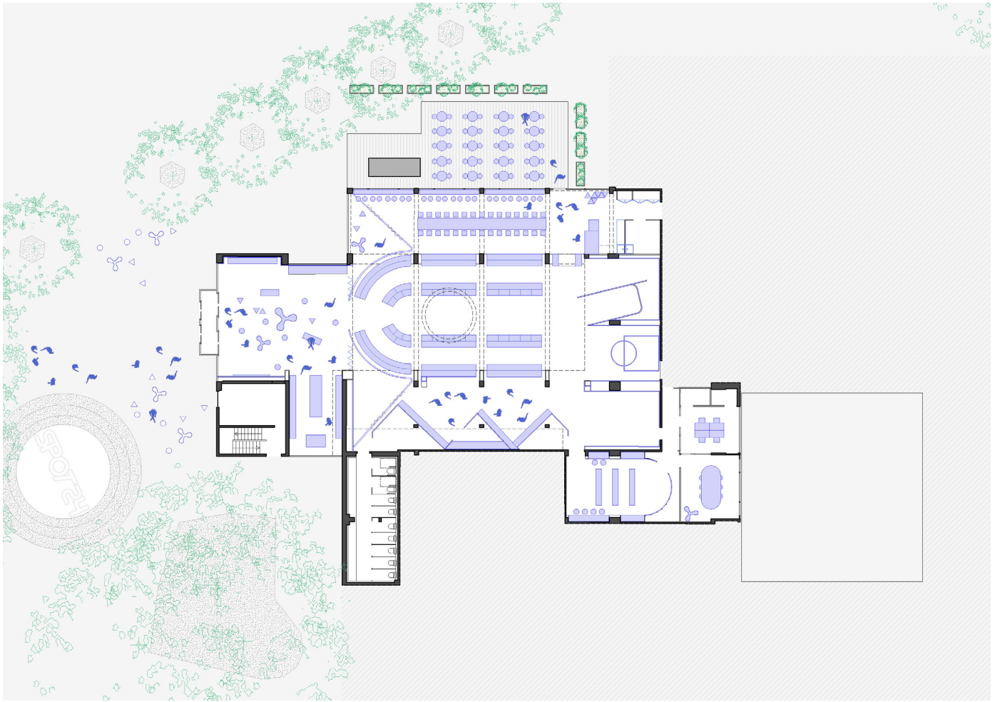
Plan du rez-de-chaussée de l'occupation temporaire, 2024 | © SAME Ground floor plan of the temporary occupation, 2024 | © SAME
