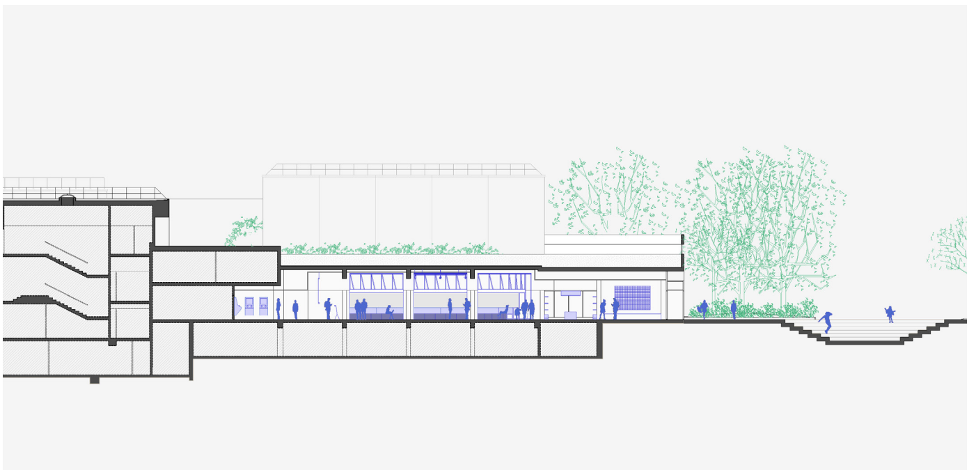
Coupe longitudinale du rez-de-chaussée de l'occupation temporaire, 2024 | © SAME Ground floor longitudinal section of the temporary occupation, 2024 | © SAME
